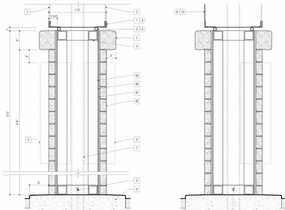
1 SETCION AT BASE - SIGN TYPE B - SIGN NO. B3 (DOUBLE FACE SIGN) SCALE: 1 1/2" = 1'-0"
