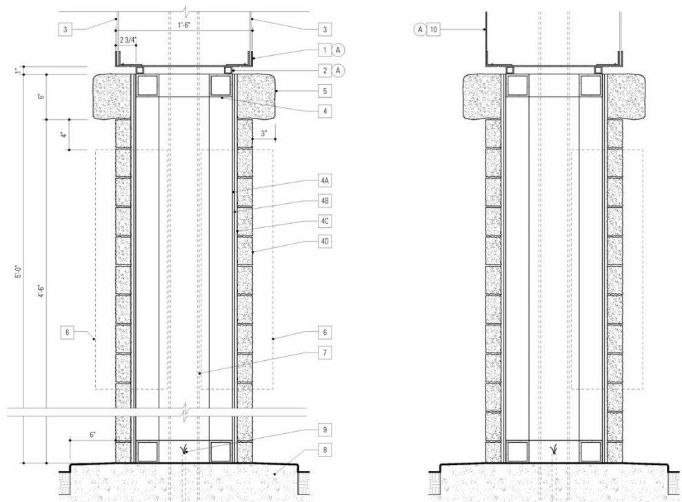
1 SECTION AT BASE - SIGN TYPE B - SIGN NO. B3 (DOUBLE FACE SIGN) SCALE: 1 1/2" = 1'-0"
